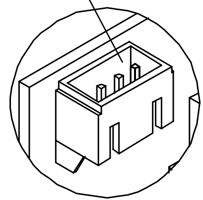
"PLUG-IN" DETAIL 1
