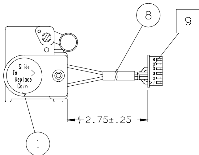
FINAL ASSEMBLY FOR 3" COILS
